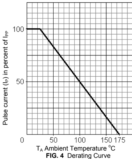
FIG. 4 - Derating Curve
